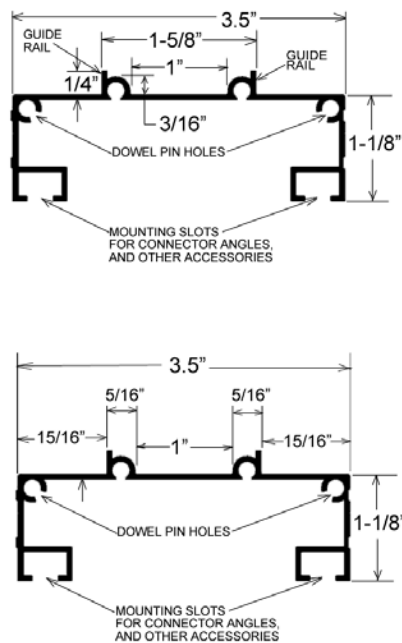
END VIEW OF SINGLE TRACK LANE
